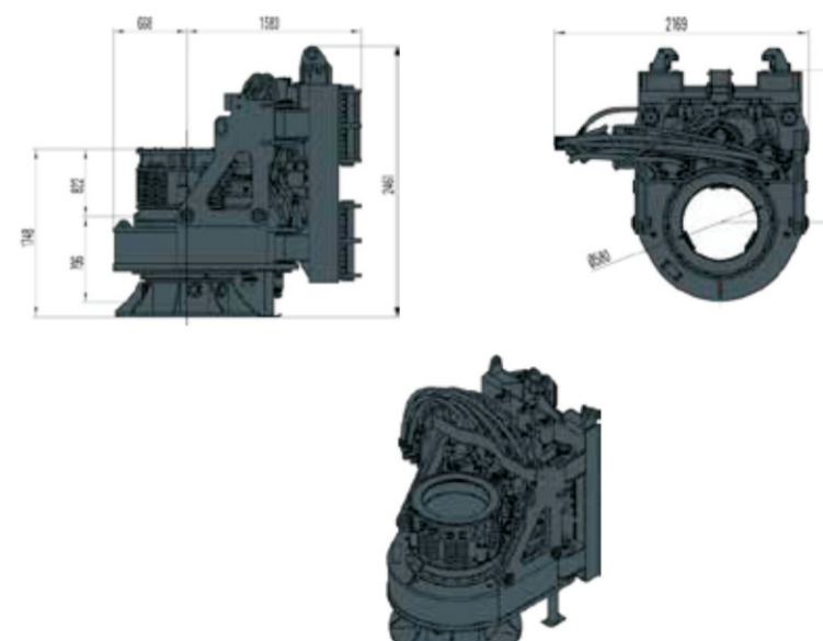
Rotary head
