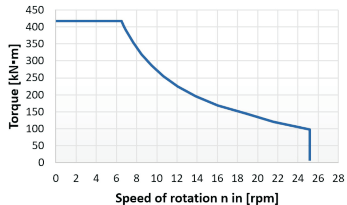
Rotary head
